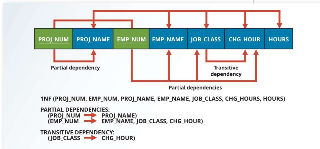
Figure 6.3 First Normal Form (1NF) Dependency Diagram
